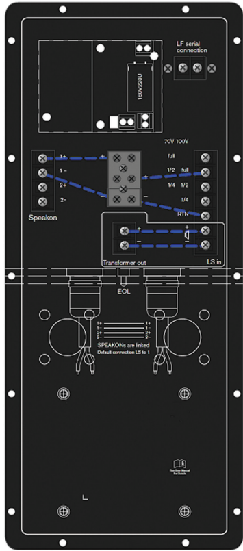
Connection panel on the rear side
