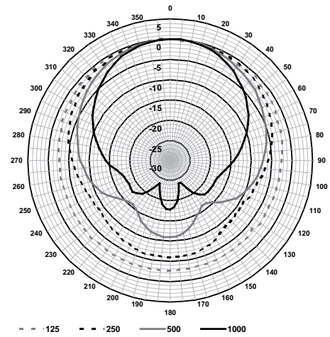
Vertical polar diagrams of LB3-PC250 (pink noise octave, normalized at 0° axis)
