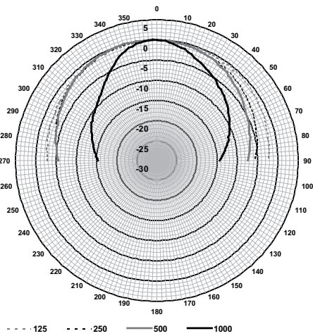
Frequency response LB3-PC250
